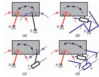
Fig. 2 Geometric constraints of some planar four-bar linkages: (a) RRRR , (b) RRPR , (c) RRRP , and (d) RRPP
