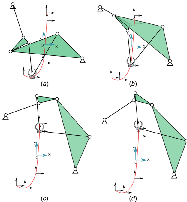
Fig. 12 Example 6.3: the sit-and-stand six-bar linkage at task positions 2, 3 (top) and 4, 5 (bottom)
