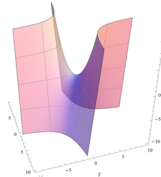
Fig. 4 A hyperbolic paraboloid defined by Z_1Z_2 - Z_3 = 0
