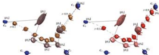
Fig. 3 (a) A rational Bézier motion of degree 6 \hat{w}_i=1+\epsilon 1 ; i=0, \dots, 3 . (b) A reparameterized rational Bézier motion \hat{w}_i=\lambda^i + \epsilon \lambda^i ; \lambda=2 and i=0, \dots, 3 .
