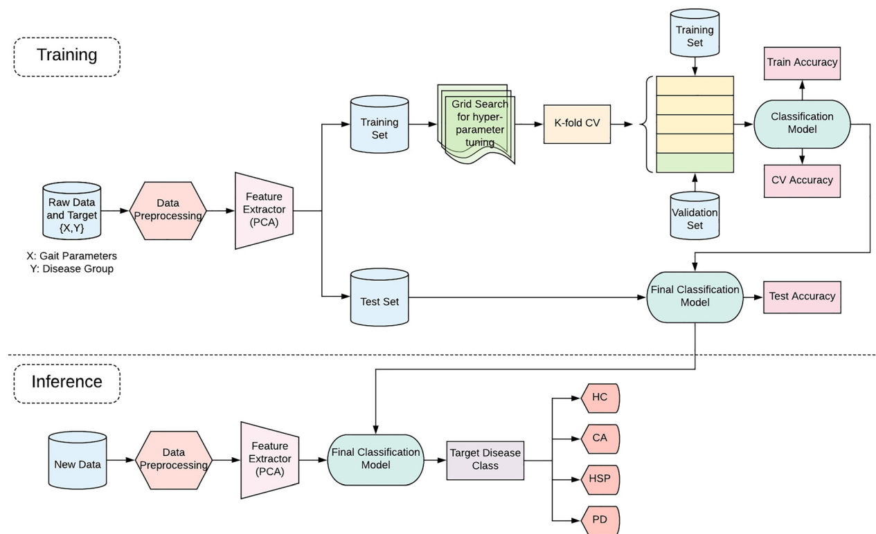
Fig. 2 Gait classification framework
