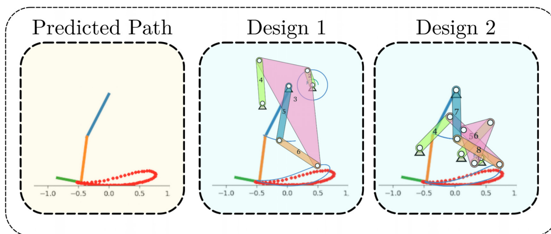
Fig. 13 Final linkage concept solutions
