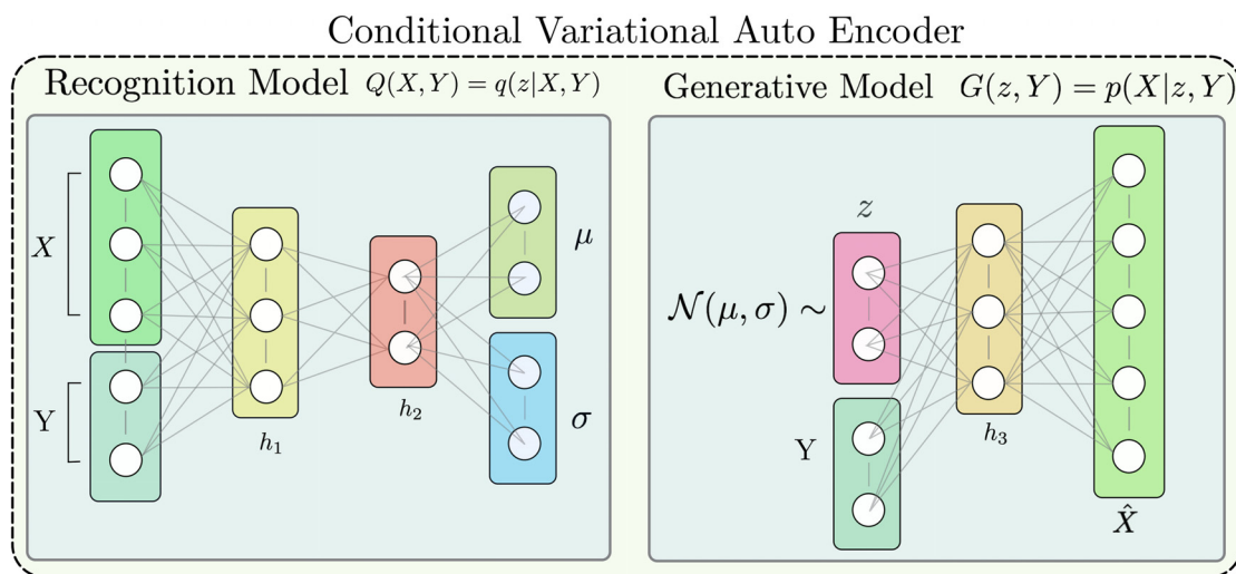
Fig. 8 Recognition model encodes the observed data X and observed property Y into probabilistic latent coding z of dimension much smaller than X . In this case, we assume a multivariate Gaussian distribution for z . Generative model takes samples from this distribution and combines it with Y to generate output \hat{X} .
