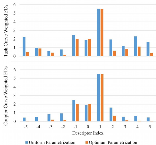
Fig. 4 Comparison of task curve and coupler curve weighted FDs for uniform and optimal parametrization
