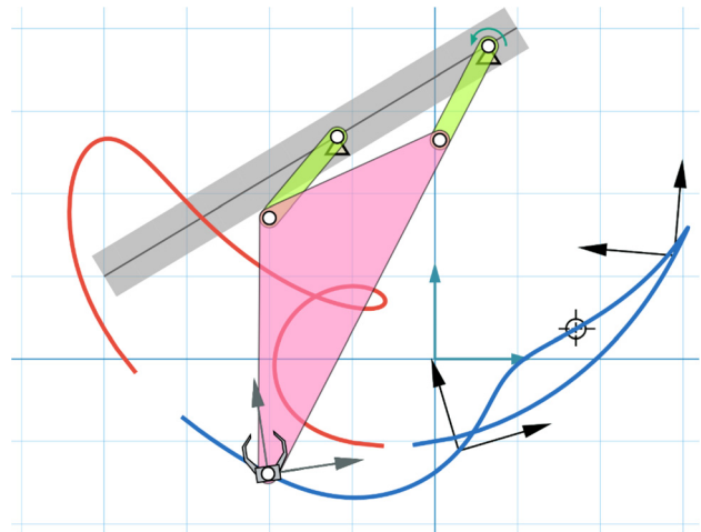
Fig. 8 Example 4: under-constrained mixed synthesis for three poses and one path points using additional motion constraint
