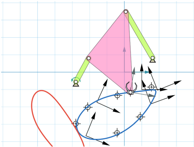
Fig. 4 Example 1: mechanism generated using mixed synthesis algorithm
