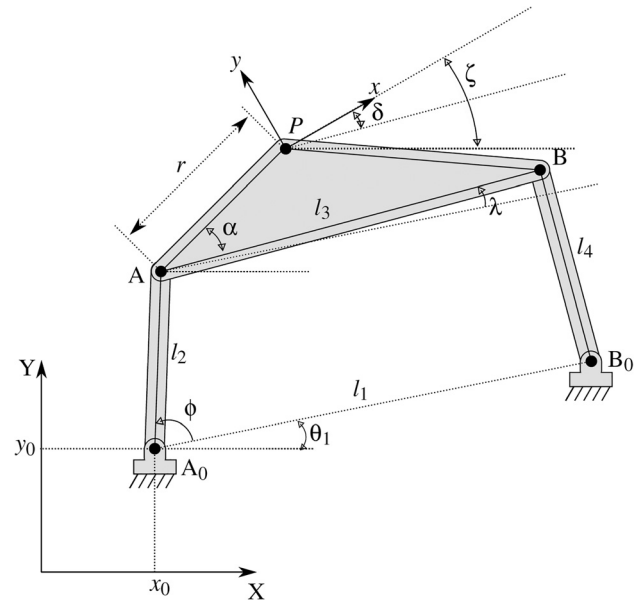
Fig. 2 Visualization of parameters describing a four-bar mechanism
