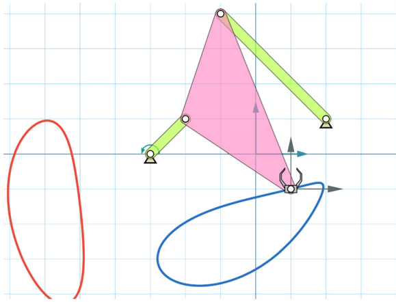
Fig. 3 Example 1: known target mechanism
