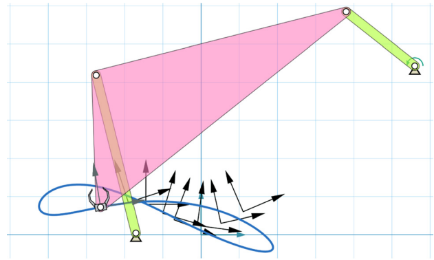
Fig. 6 Example 2: over-constrained motion synthesis for eight poses produces a poor solution
