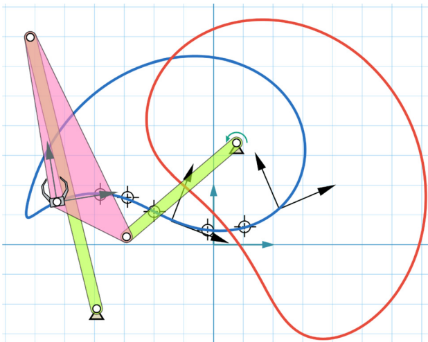
Fig. 5 Example 2: mixed synthesis with fully constrained MSP computation for three poses and five path points
