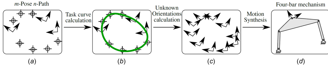
Fig. 1 An overview of our approach to the Alt-Burmester problems: (a) specify m -pose, n -path points, (b) a task curve is fit through the m + n path points using Fourier series, (c) use the harmonic content of the path data to find the missing orientations at the n -path points, and (d) finally, compute both type and dimensions of planar four-bar linkages
