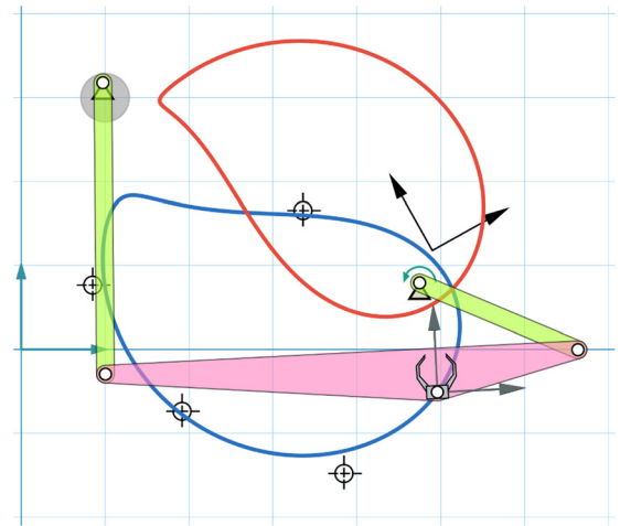
Fig. 7 Example 3: under-constrained mixed synthesis for two poses and four path points using additional mixed constraint
