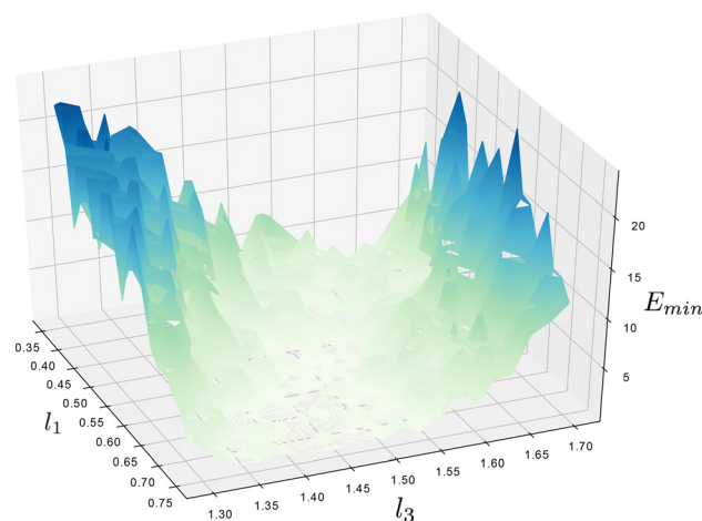
Fig. 14 Distance ( E_{min} ) from Eq. (4) as the parameters l_1 and l_3 are varied. Although open loop breaks at l_1 :0.55, l_3 :1.5, there are no spikes of error function in the region near singularity, as the shape is very similar between the two topologies.
