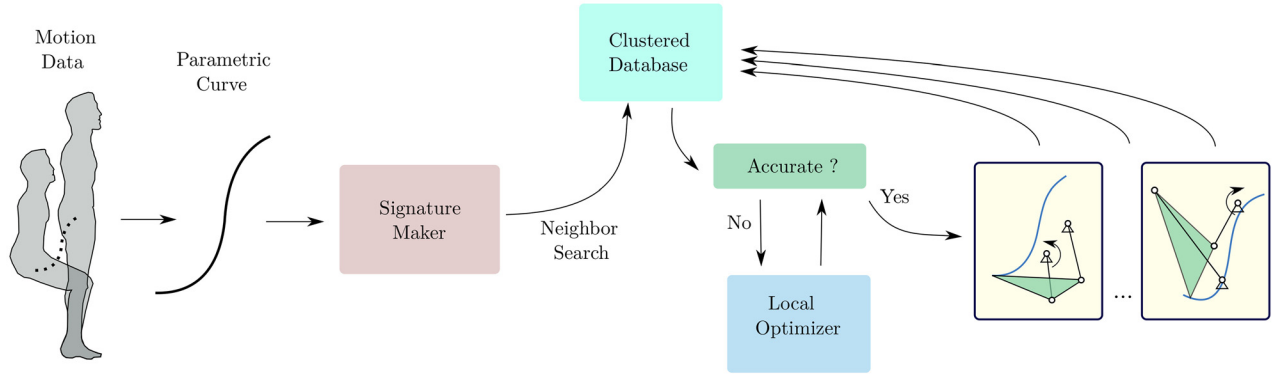
Fig. 2 The machine learning approach begins by creating an invariant signature for the path and the motion data, which facilitates a compact and hierarchical clustered database and an auto-encoder neural network trained to elicit good, defect-free solutions or subjected to local, fast optimization. The results are defect-free conceptual design solutions for input problems.
