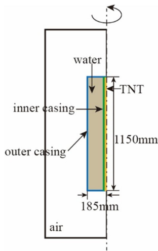
Fig. 14 Schematic of the computational model
