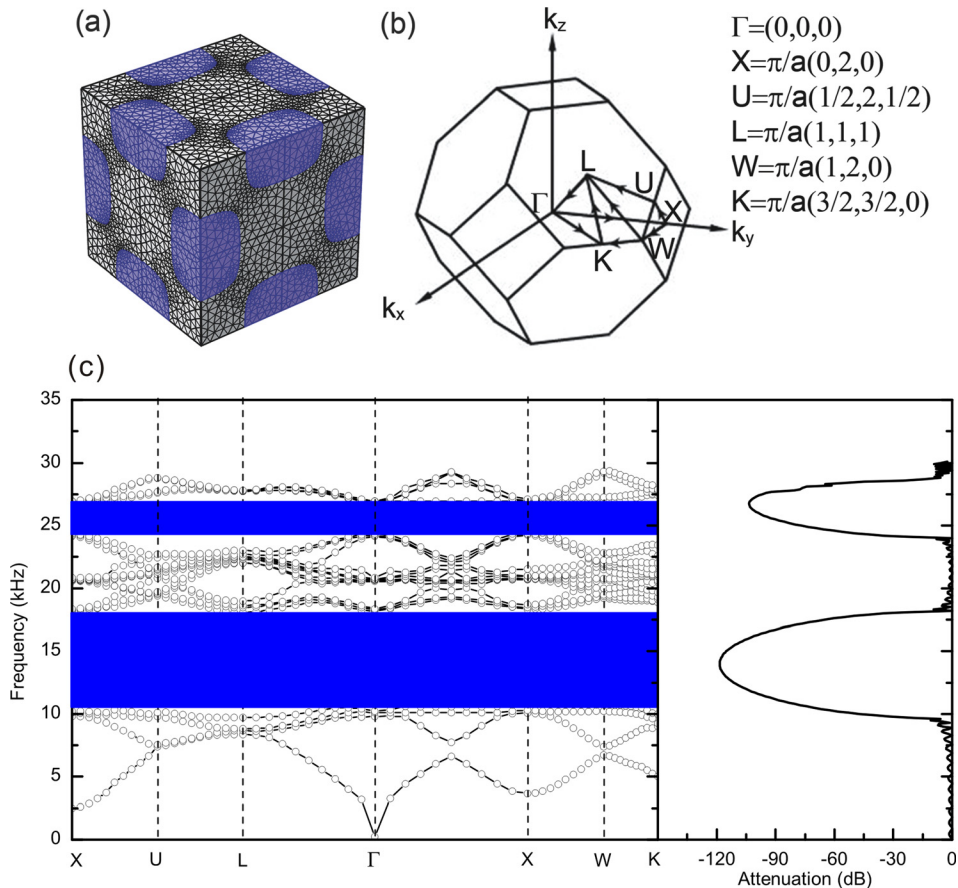
FIG. 8. (a) The unit cell of face-centered cubic lattice in FEM, (b) the first irreducible Brillouin zone of face-centered cubic lattice and (c) the band structure and sound attenuation along \Gamma X at the volume fraction of 0.54.
