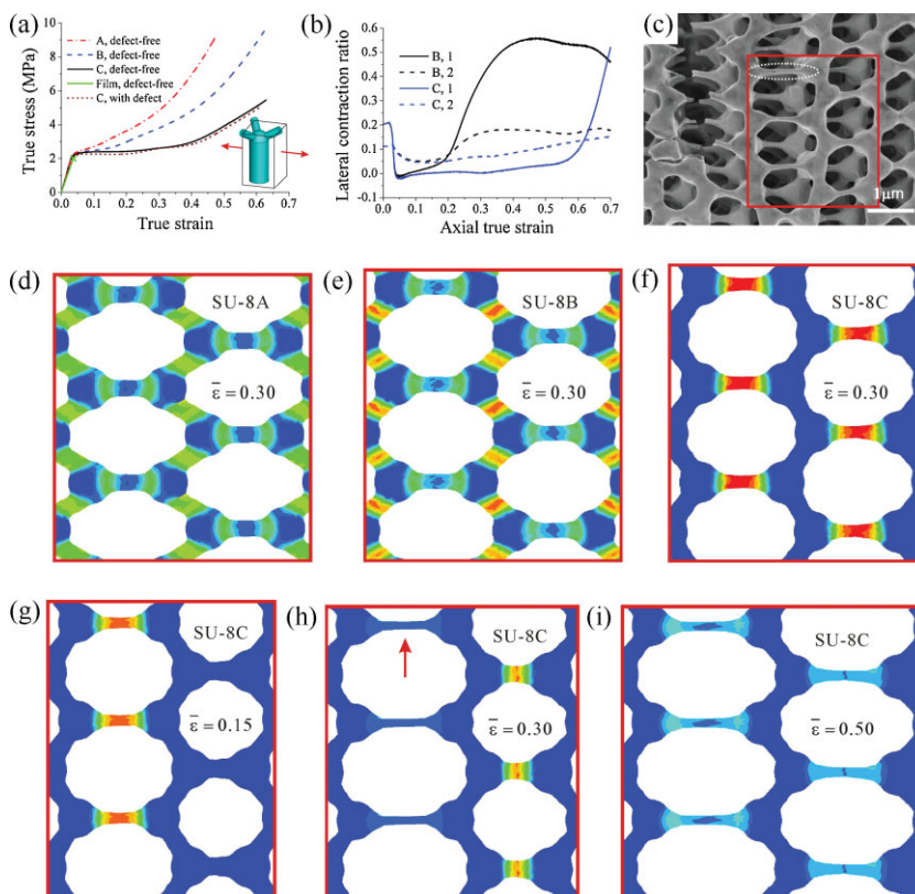
Figure 3. Mechanical response of microframe structures under macroscopic uniaxial tension in the 3-direction. a) Macroscopic true stress–strain curves of defect-free and imperfect microframe structure with various material properties. b) Lateral contraction ratios versus axial true strain using material property SU-8B and SU-8C. c) Experimental evidence of plastic deformation of structural elements with up to 300% plastic strain (e.g., circled beam) [12]. d–f) Simulated micrograph of defect-free microframe structure at a strain of 0.30 using material property SU-8A, SU-8B, and SU-8C, respectively. g–i) Simulated micrographs of microframe structure with imperfections at strains of 0.15, 0.30, and 0.50, where beam (pointed out) strain is about 280%. The progression in strain is in agreement with the experimental observations as depicted in the SEM image (Fig. 3c).
