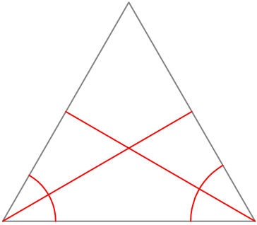
Draw bisectors
