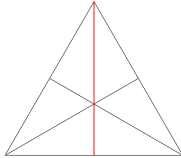
Connect bisectors
