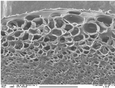
Figure 2. EVA 350 @ ~ 1100 psi Under SC conditions (100x)
