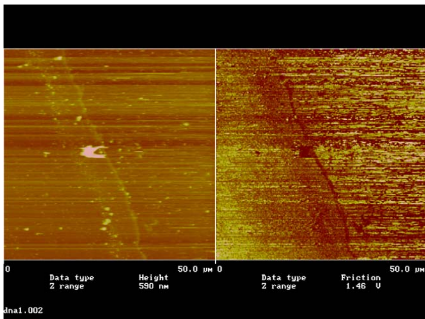
Atomic Force Microscopy (AFM) images in topological (left) and friction (right) mode of adsorbed DNA ring on Octadecyltrichlorosilane-covered Si surface
