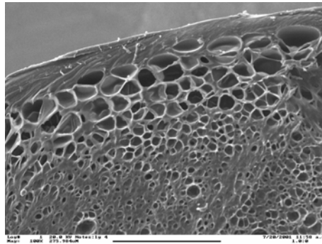
Figure 3. EVA 350 @ ~ 2500 psi Under SC conditions (100x)
