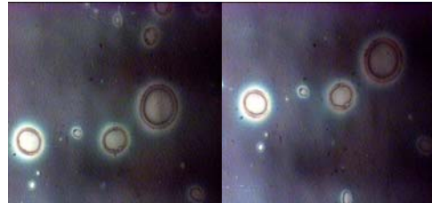
Figure 2- 58K PMMA (under 100x magnification) first after 30 minutes of annealing at 165^\circ\text{C} and then after 50 minutes of annealing. Dewetting proceeds much slower at this higher molecular weight
