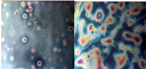
Figure 1- 4K PMMA (under 50x magnification) first after 15 minutes of annealing at 165^\circ\text{C} and then after 22 minutes of annealing. After 22 minutes dewetting is already complete
