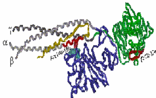
Fig. 2: Structure of fibrinogen
