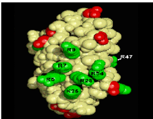
Fig. 1: Heparin binding cradle
