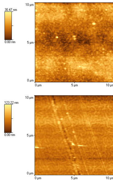
Figure 2: AFM scans- sputtered 30 mg/mL di-block copolymer film on Si [top] sputtered surface
