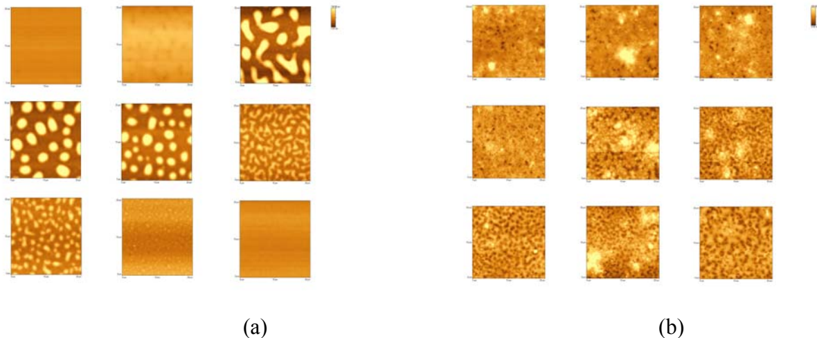
Figure 1. In each of the 20\mu\text{m}\times 20\mu\text{m} AFM topographical picture above, from top left to lower right, ratio of PS to PMMA changes from 90:10 to 10:90, the amount of PMMA increases by 10% each time. (a) PS/PMMA thin films without clay added. (b) In each thin film, there is 10% by weight of Cloisite 6a added.
