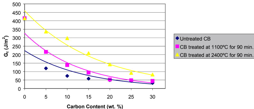
Fracture Toughness of PS/PS with Carbon Black at the Interface
