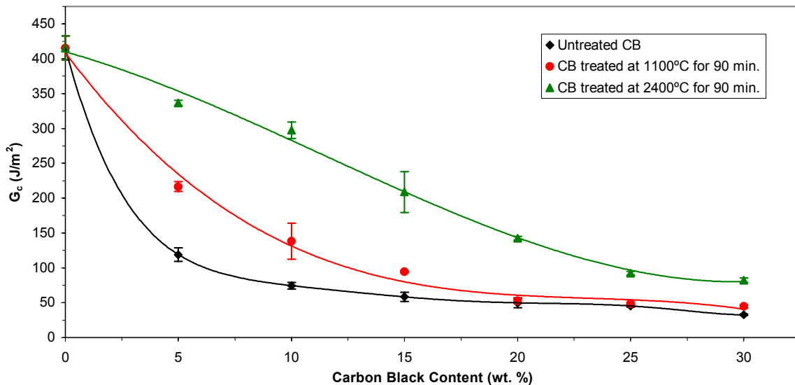
Fracture Toughness of PS/PS with Carbon Black at the Interface
