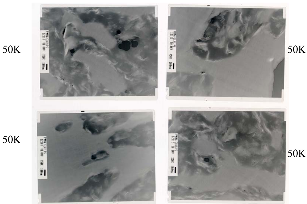
TEM Images of PMMA+PS+CLAY (45/45/10wt%)
