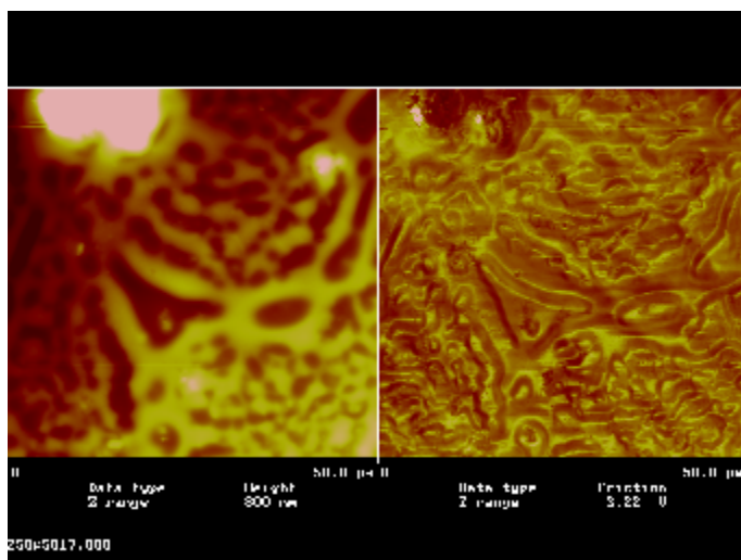
50% Polycarbonate and 50% Styrene Acrylonitrile-17 with 5% Cloisite 20A
