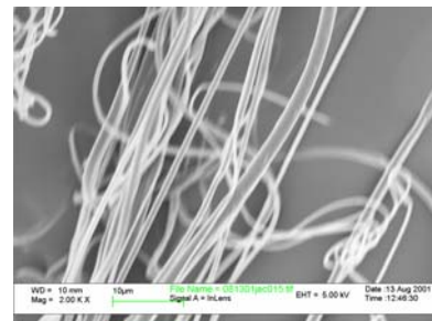
Polypropylene treated at 1100 psi at 96 °F viewed under the SEM.
