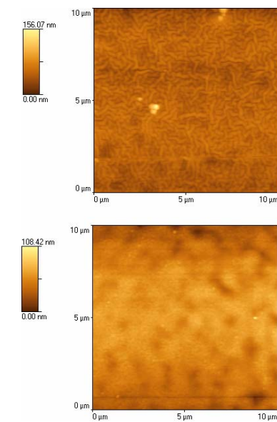
Figure 1: AFM scans- sputtered 15 mg/mL di-block copolymer film on Si [top] un- sputtered surface [bottom]
