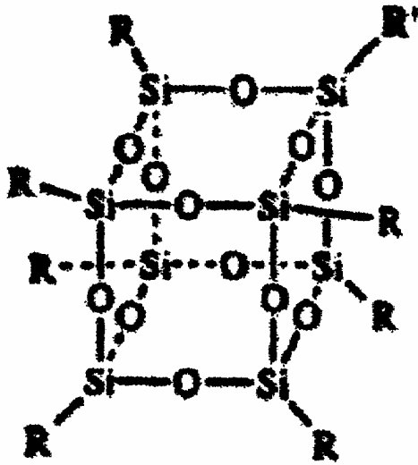
Figure 1 - Chemical Structure of POSS
