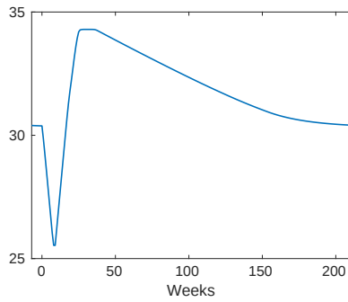
(e) Debt
