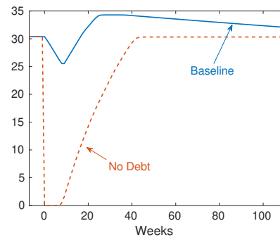
(h) Debt
