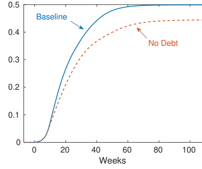
(b) Deceased
