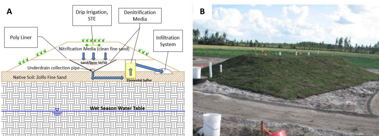
Figure 3. A) Simplified schematic of a FOSNRS design (modified from Anderson and Hirst, 2015b; Hazen and Sawyer, 2015). B) Photograph of final installation.
