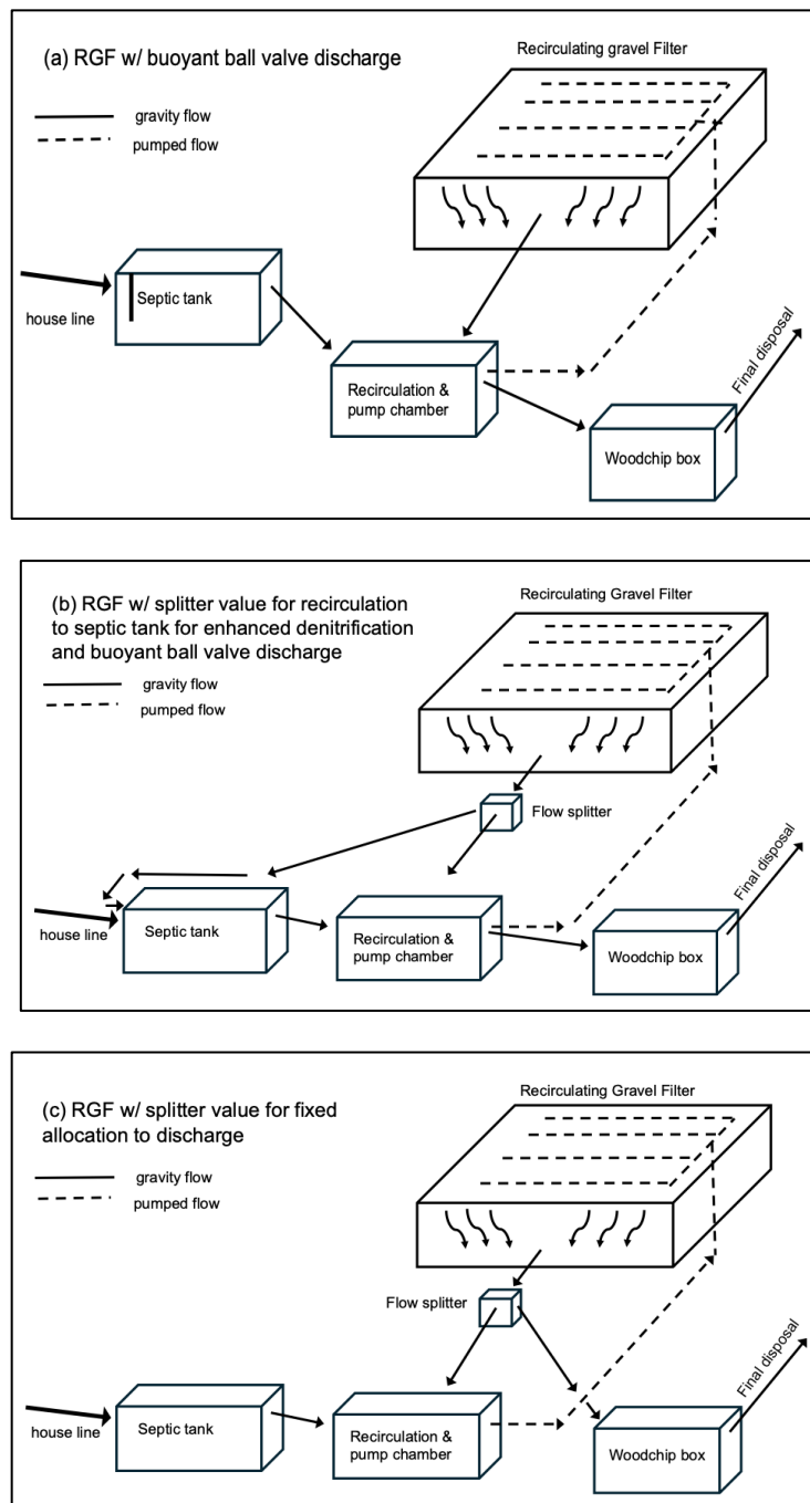
Fig. 1. Flow schematics of (a) recirculating gravel filter (RGF) coupled to a woodchip biofilter (WCB) with effluent discharge by buoyant ball valve located in recirculation & pump chamber; (b) RGF with flow splitter to septic tank to enhance denitrification capacity and effluent discharge by buoyant ball valve located in recirculation & pump effluent chamber and (c) RGF with effluent discharge of fixed % of flow at flow splitter. With fixed % discharge, pump controls must include a redundant off switch to prevent pump from overheating during no flow conditions.
