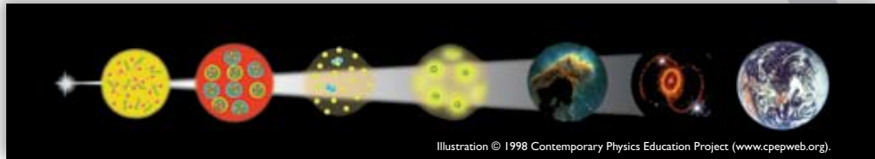
Illustration © 1998 Contemporary Physics Education Project ( www.cpepweb.org ).
